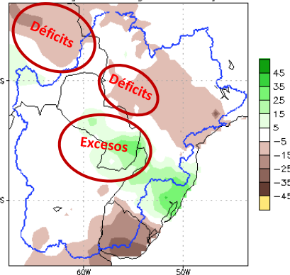
NCEP GFS Ensemble Forecast 8-14 Day Precipitation (mm) from: 17Aug2025 for La Plata_Basin 24Aug2025-30Aug2025 Anomaly
