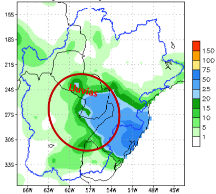
NCEP GFS Ensemble Forecast 8-14 Day Precipitation (mm) from: 17Aug2025 for La Plata_Basin 24Aug2025-30Aug2025 Accumulation
