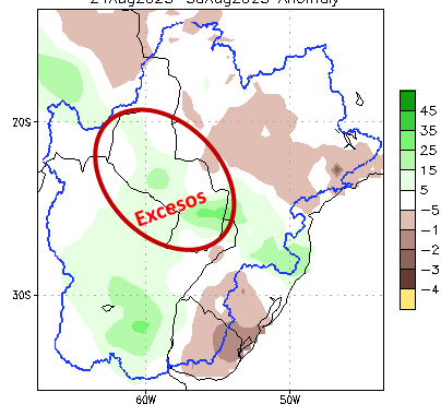
NCEP GFS Ensemble Forecast 1–7 Day Precipitation (mm) from: 24Aug2025 for La_Plata_Basin 24Aug2025–30Aug2025 Anomaly
